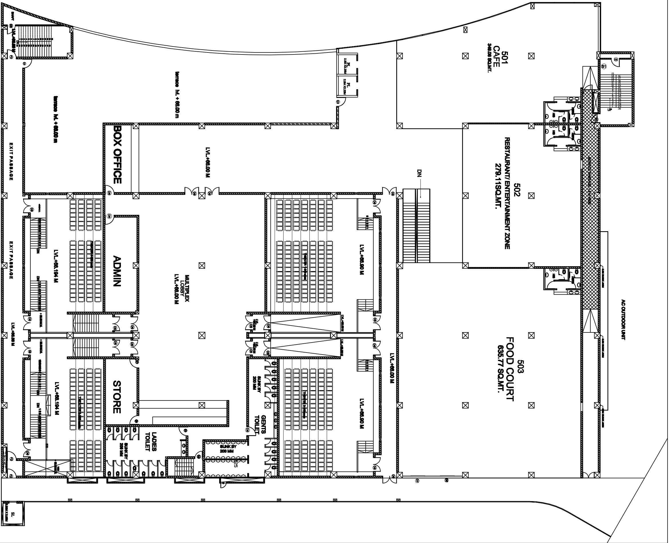
FOURTH FLOOR PLAN
